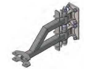
Base part heavy hook 90° raised
